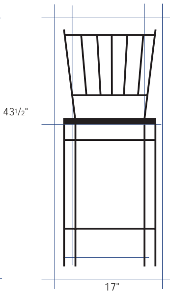
Wood Slatback Stool BS627
